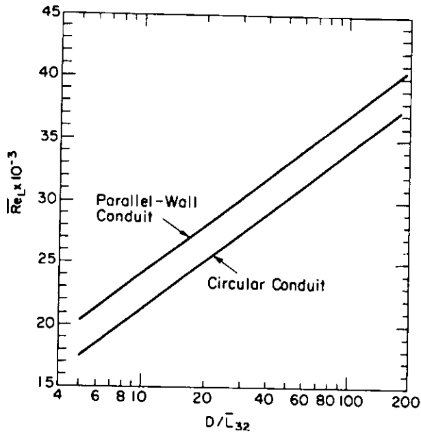
Fig. 4. The predicted relation between the (mean velocity in conduit) \times (mean scallop size) Reynolds number ( \overline{Re}_L ) and the ratio of conduit diameter or width to mean scallop size ( D/\overline{L}_{32} ).
